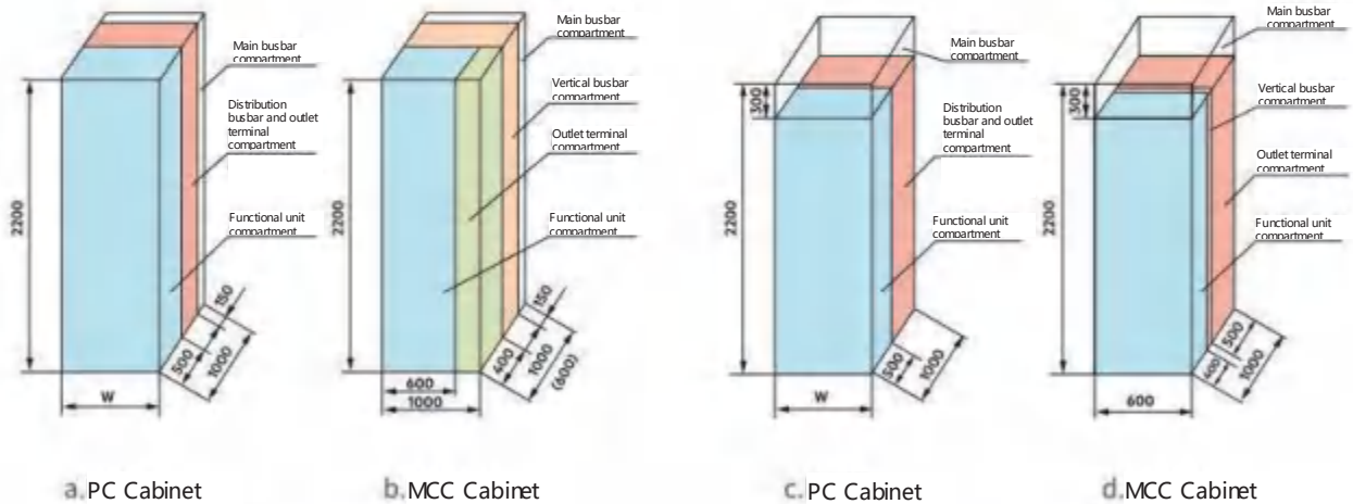
MLS structure (rear-mounted busbar)
